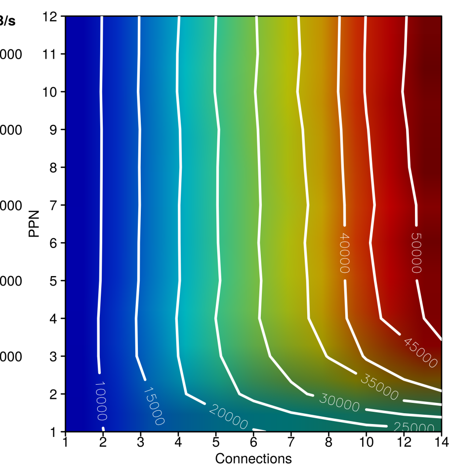
Fig. 3: Granularity: 100 KB
