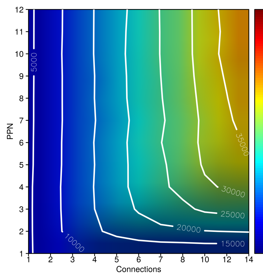
Fig. 2: Granularity: 16 KiB
