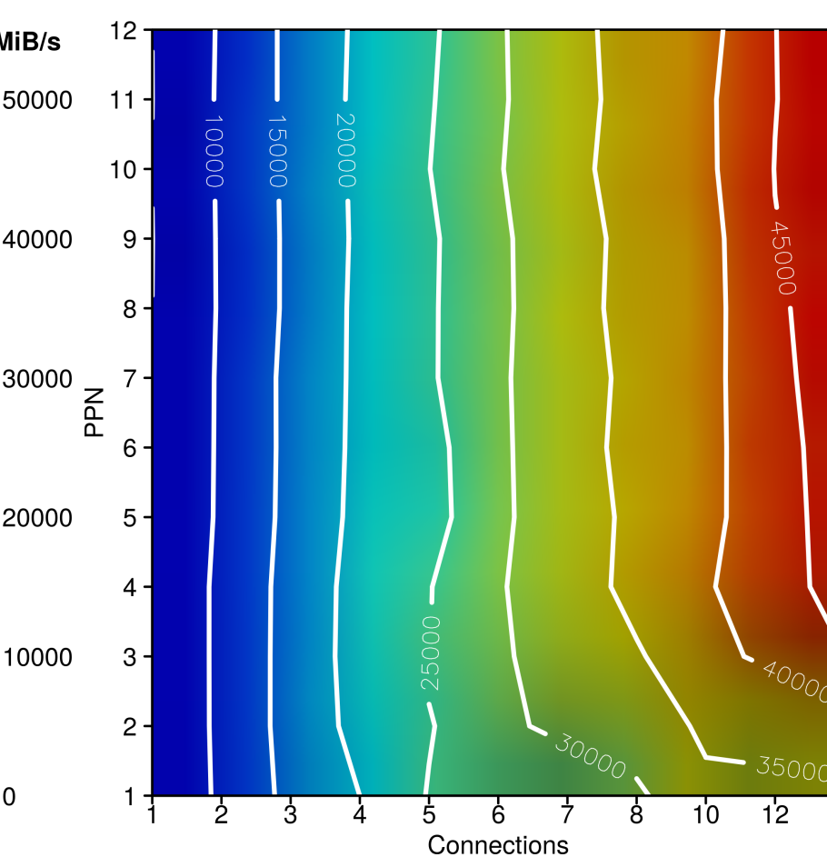
Fig. 4: Granularity: 10 MiB
